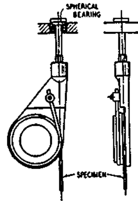
FIG. 37 Snubbing-Type Gripping Device
