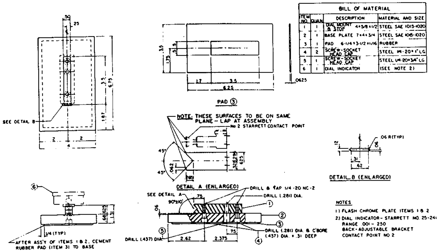
FIG. 16 Assembly and Details for Lateral Expansion Gauge
