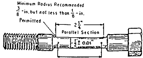
FIG. 33 Tension Test Specimen for Bolt with Turned-Down Shank
