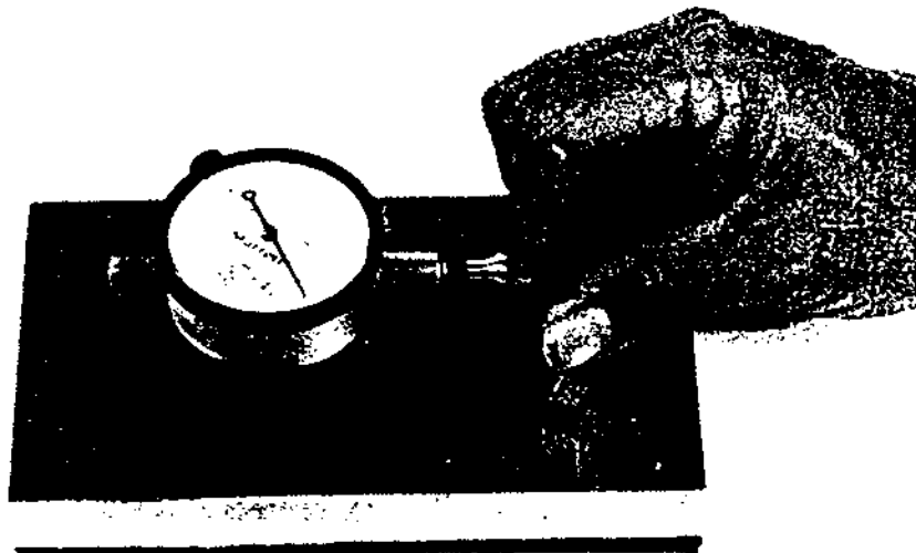
FIG. 15 Lateral Expansion Gage for Charpy Impact Specimens
