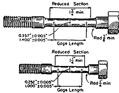
FIG. 34 Examples of Small Size Specimens Proportional to Standard 2-in. Gage Length Specimen
