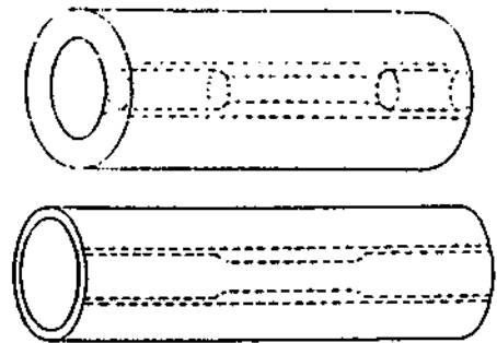
FIG. 18 Location of Strip Tension Test Specimens in Large Diameter Tubing
