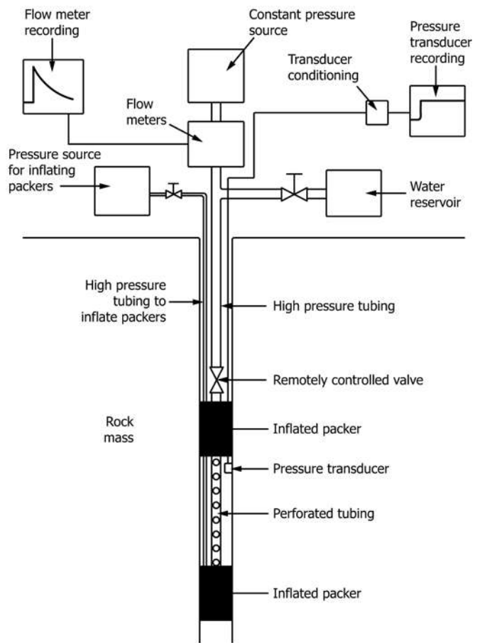
FIG. 1 Equipment Schematic
