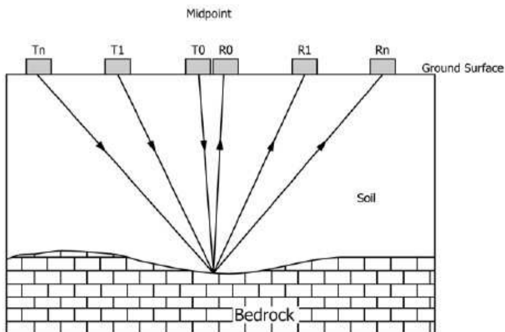
FIG. 5 Schematic Diagram of a Common Midpoint (CMP) Sounding Order # FOR OFFICIAL USE not FOR SALE/Downloaded: 2016-01-12 Single-user licence only, copying and networking prohibited.
