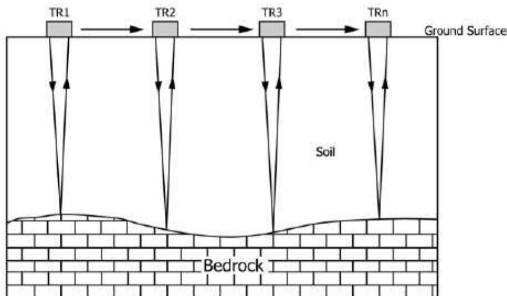
FIG. 4 Schematic Diagram of the Reflection Profiling Method Order # FOR OFFICIAL USE not FOR SALE/Downloaded: 2016-01-12 Single-user licence only, copying and networking prohibited.
