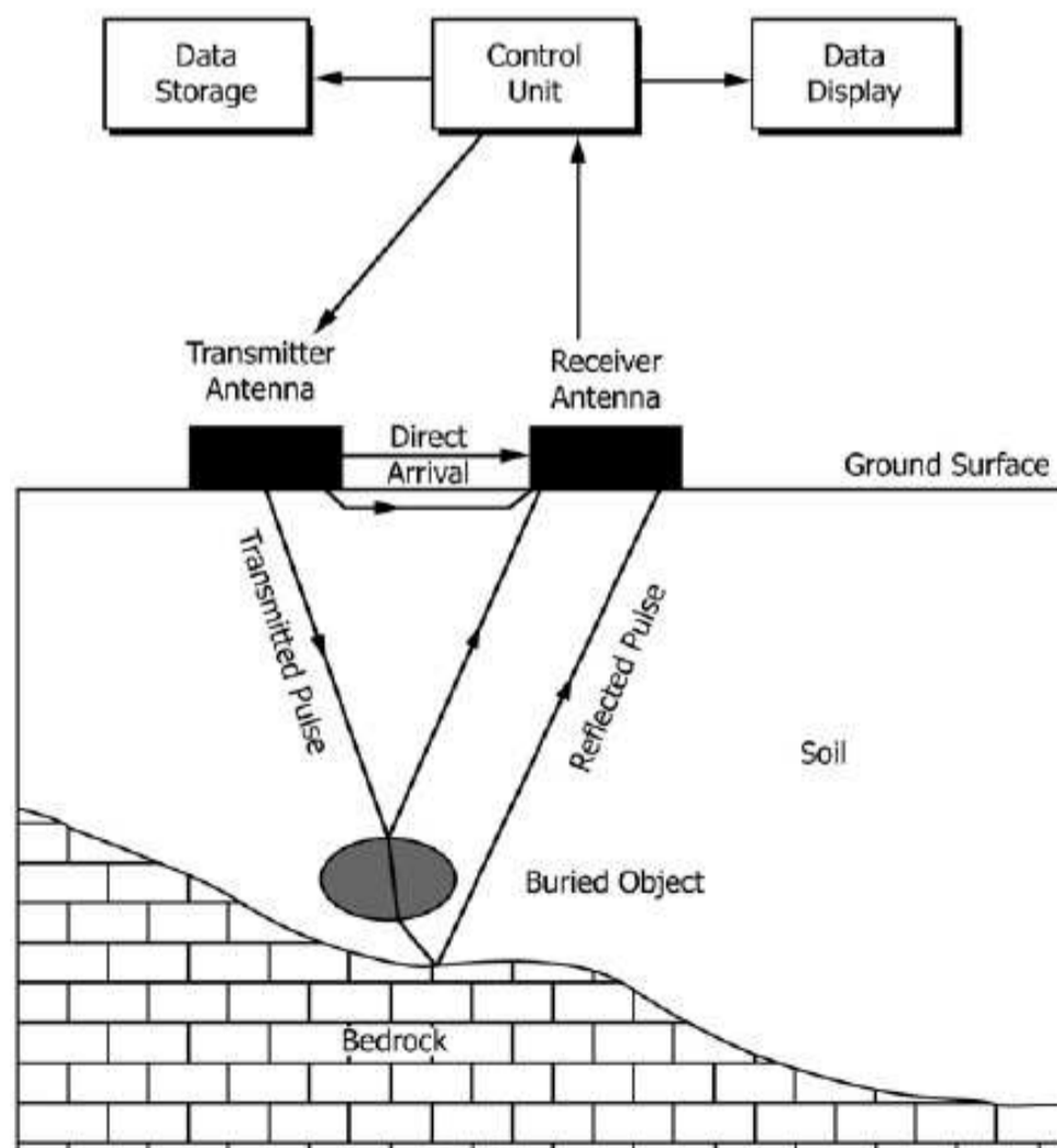
FIG. 1 Schematic Diagram of a Ground Penetrating Radar System Order # FOR OFFICIAL USE not FOR SALE/Downloaded: 2016-01-12 Single-user licence only, copying and networking prohibited.
