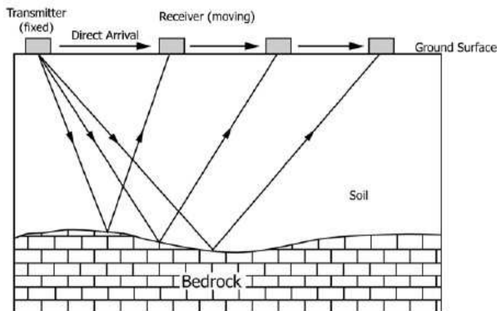
FIG. 6 Schematic Diagram Showing a Wide Angle Reflection Sounding
