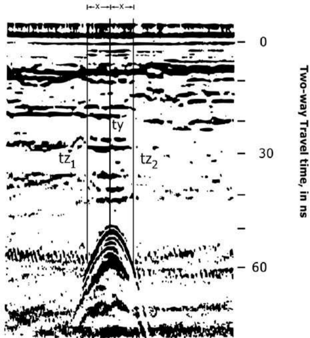
FIG. 3 Generalized Diagram of a Pipe Signature: GPR Record (300 MHz) Showing a Hyperbola from a Buried Pipe, and Computation of Depth and Velocity from that Target (see 6.7.2.3(2b))
